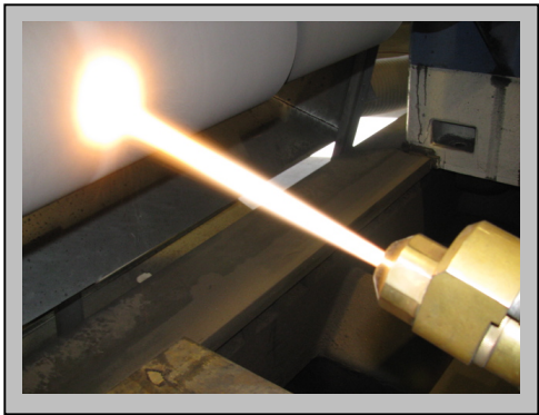
Close-up of HVOF Spray Process On Hydraulic Cylinder Rod
