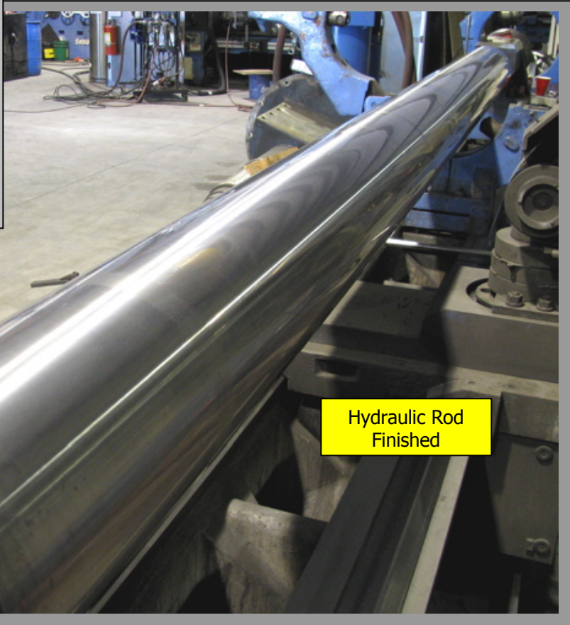
Hydraulic Rod After HVOF Coating Applied
